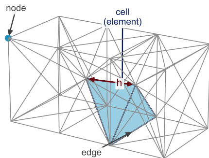
(e) Tetrahedral mesh (3D)
