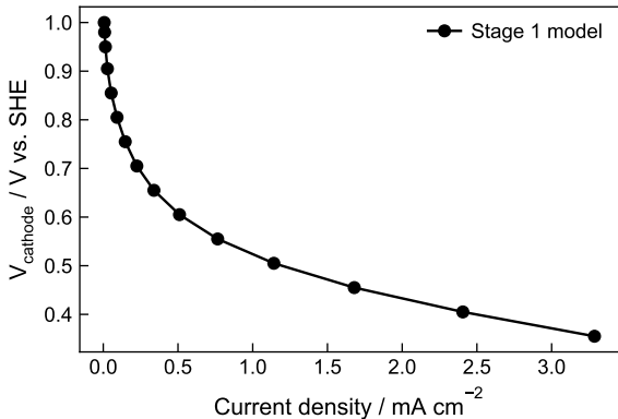
Stage 1 polarization curve
