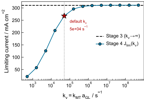
Limiting current vs interphase rate
