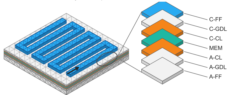
Model layout: serpentine flow field on the MEA
