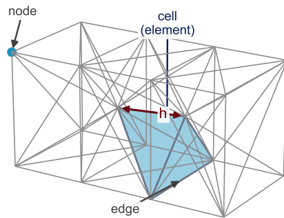
(e) Tetrahedral mesh (3D)
