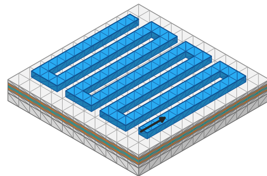
(f) Model layout: serpentine flow field on the MEA
