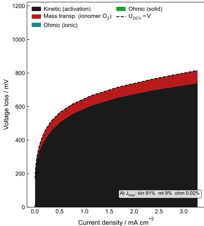
(a) Stage 1 applied-voltage breakdown
