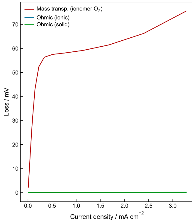
(b) Non-kinetic losses
