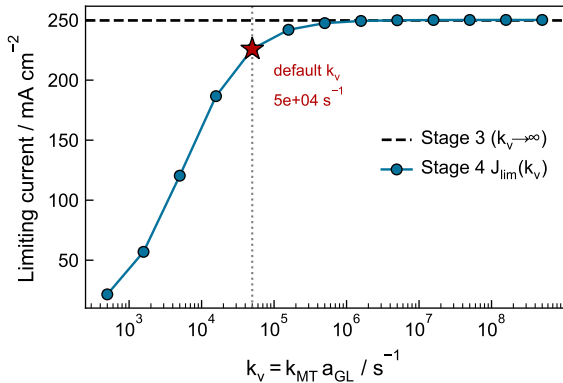
Limiting current vs interphase rate
