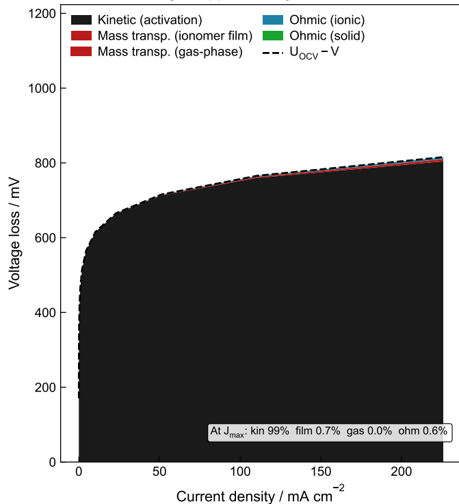
(a) Stage 4 applied-voltage breakdown
