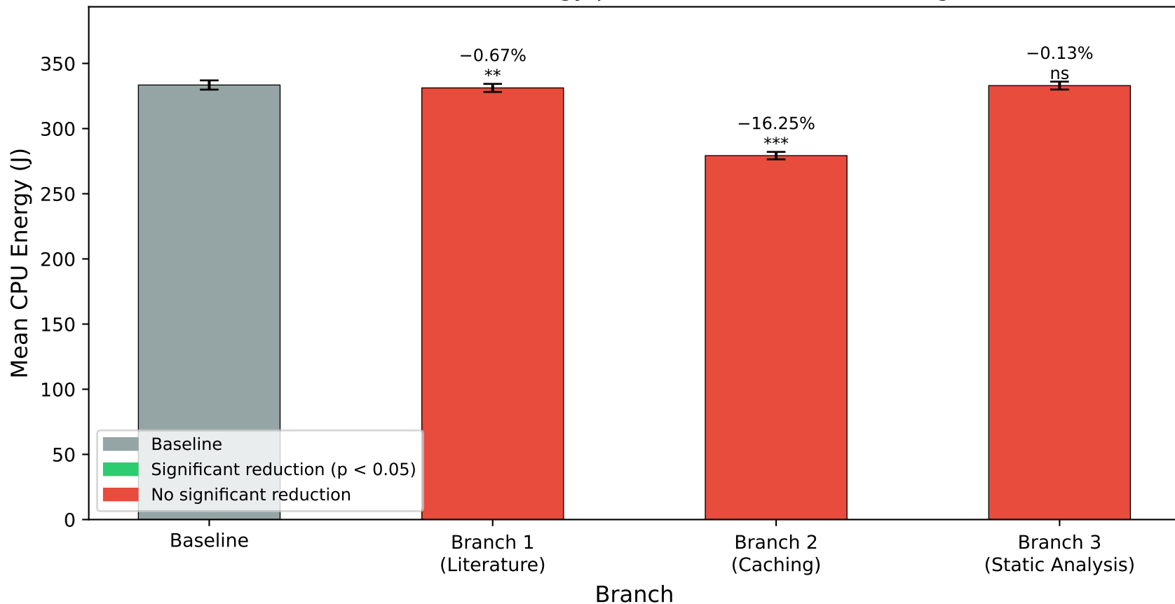
RQ2 — Mean CPU Energy per Branch (Individual Changes)
