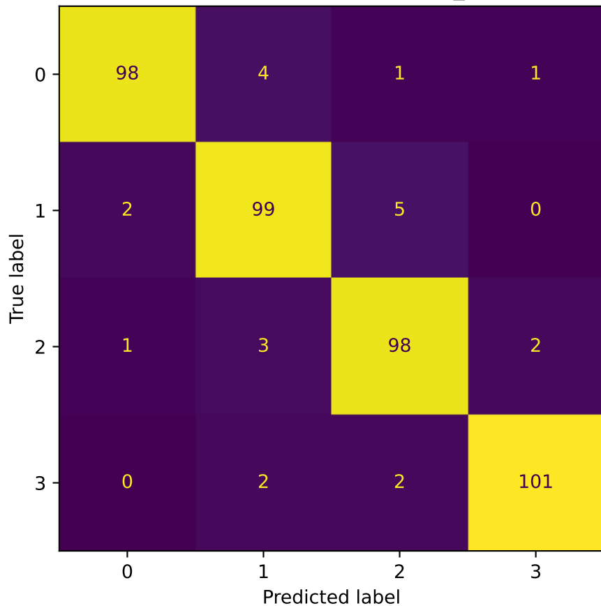
OOF confusion matrix: gradient_boosting
