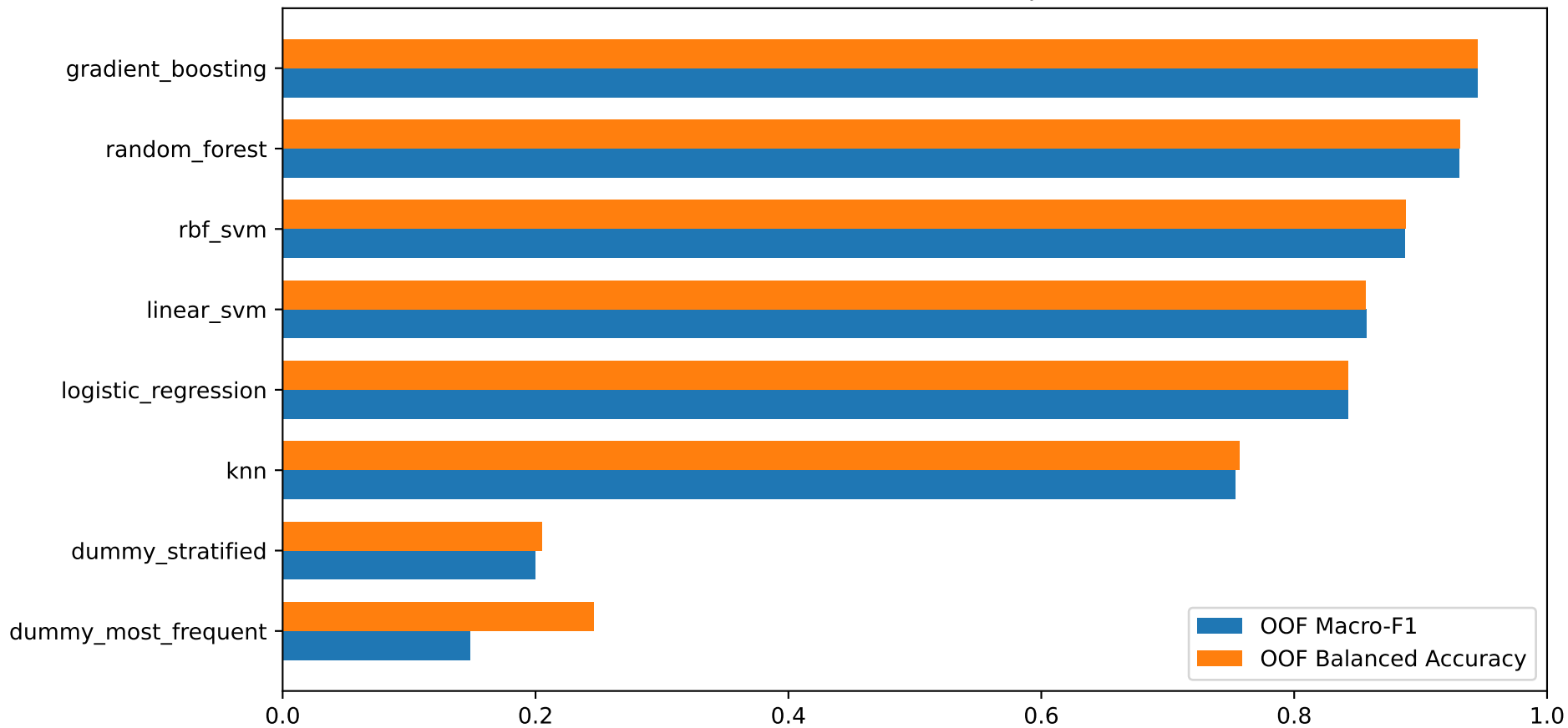
Traditional baseline comparison
