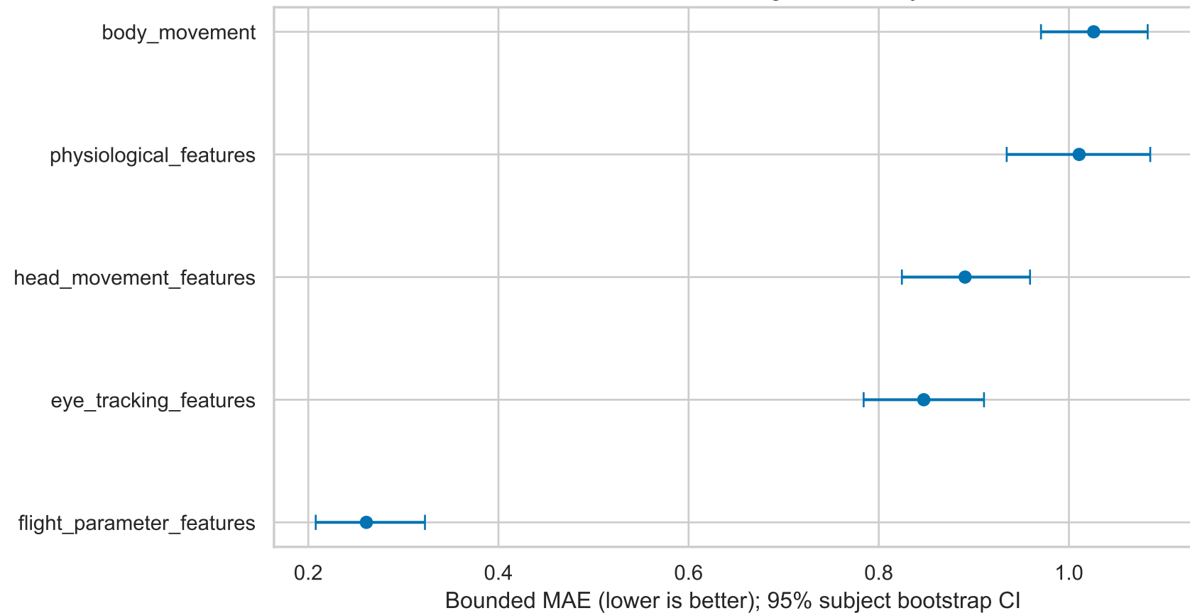
Phase 07 unimodal ranking — n=35 subjects
