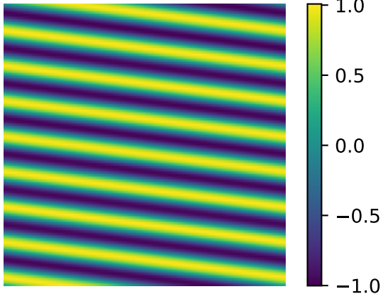
Predicted u(x,t)
