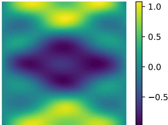
Predicted u(x,t)
