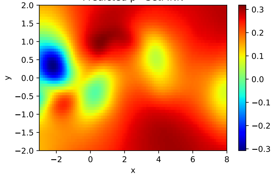
Predicted p - SetPINN
