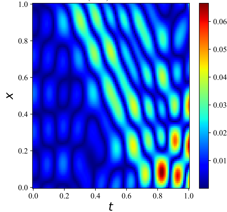
1D Wave (FLS) - Absolute Error
