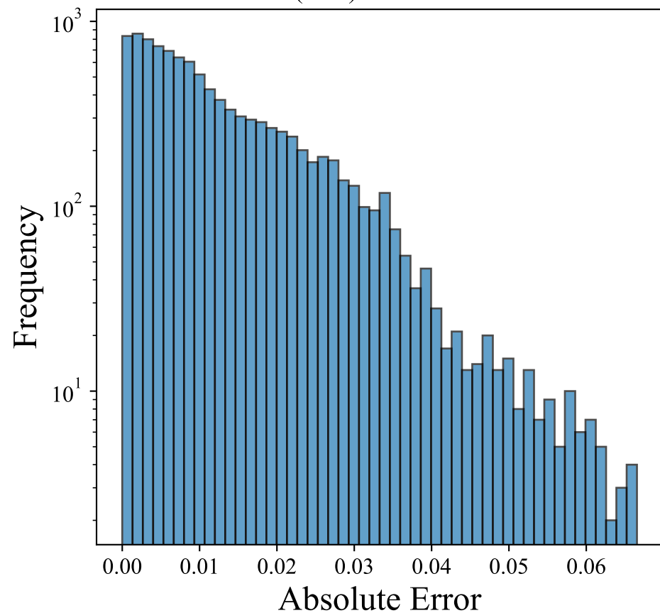
1D Wave (FLS) - Error Distribution
