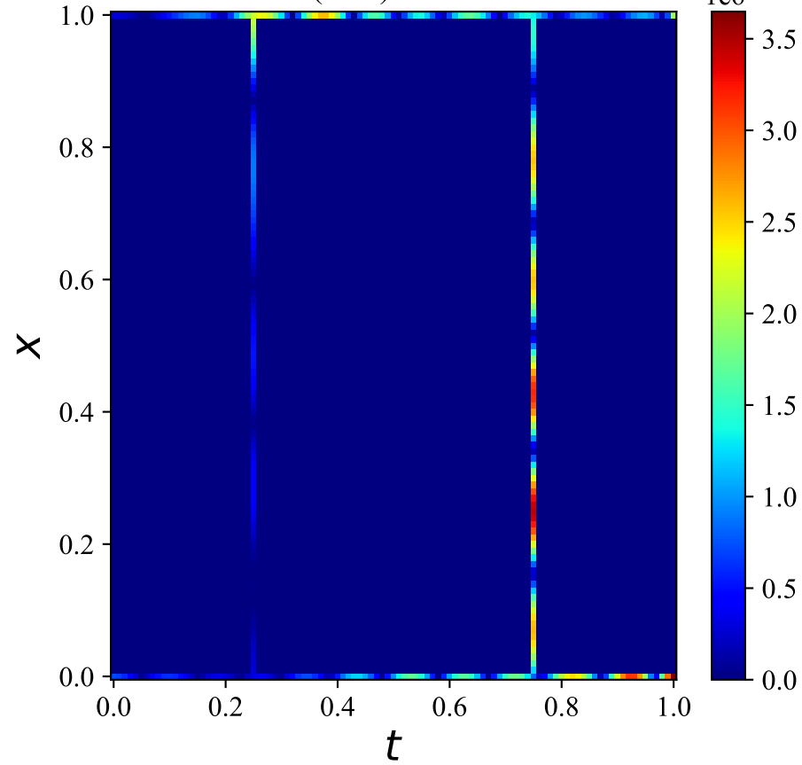
1D Wave (FLS) - Relative Error
