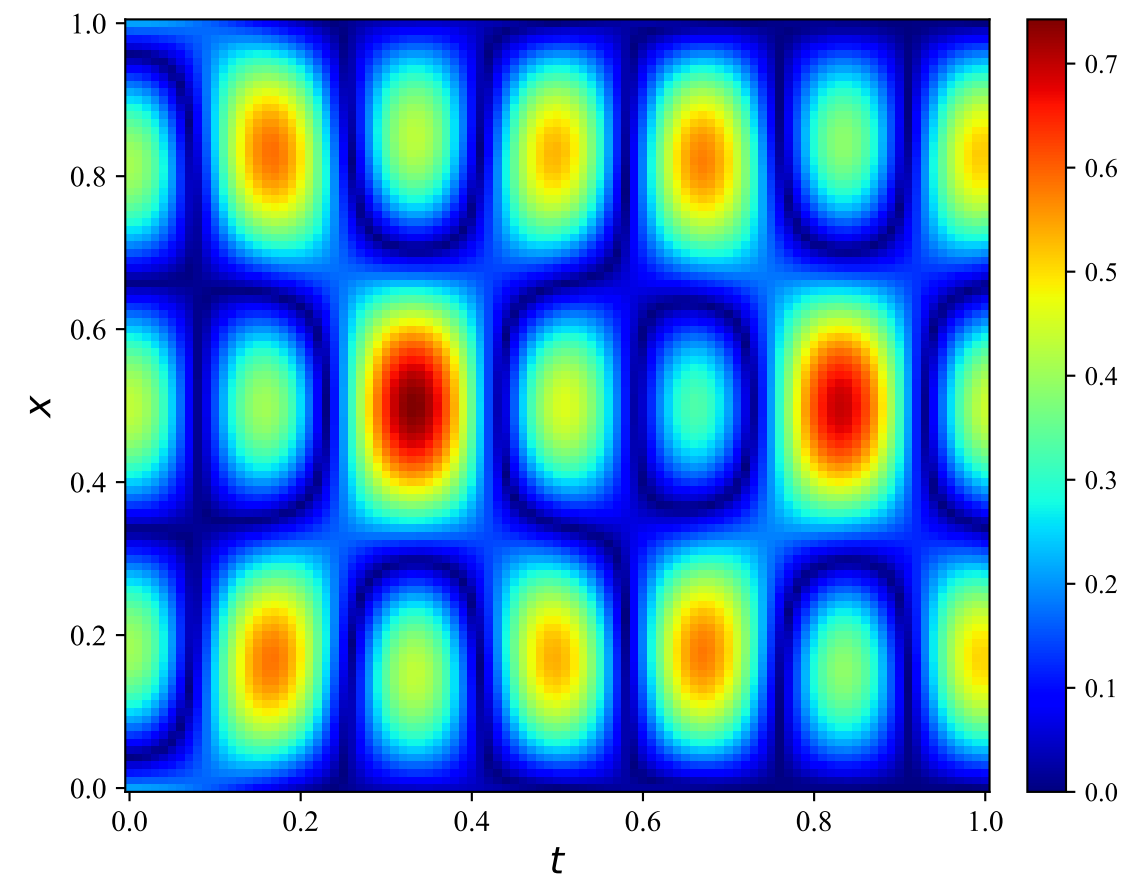
PINNsFormer
