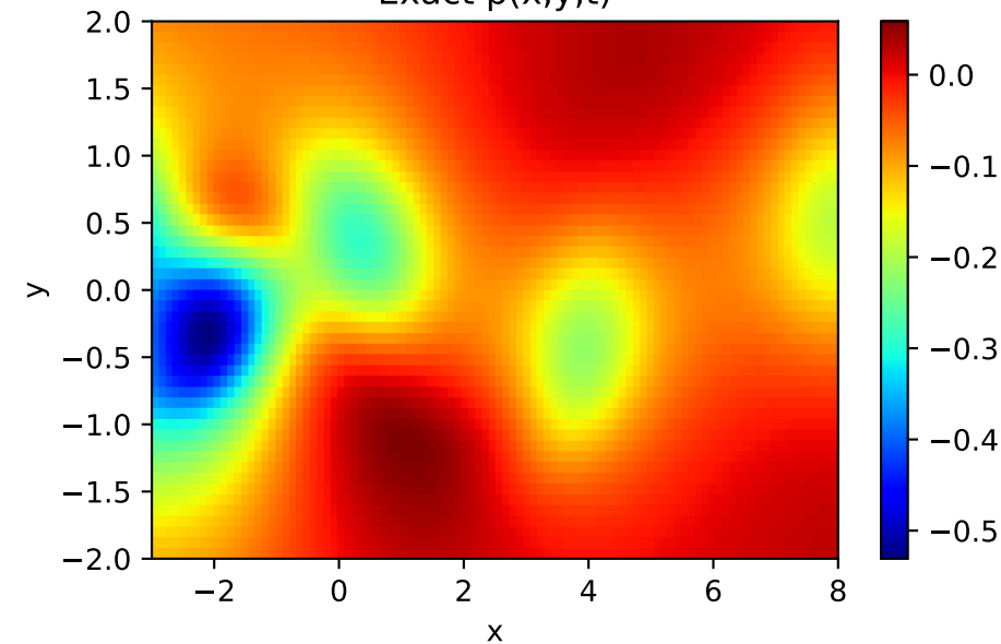
Exact p(x,y,t)
