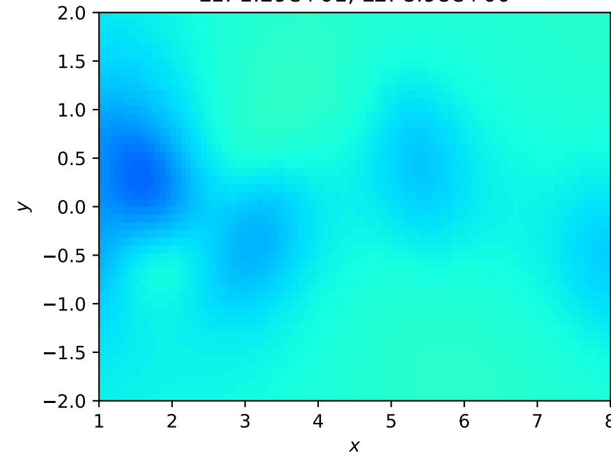
NS Pressure Error (PINNsFormer_Enc_Only) L1: 1.29e+01, L2: 8.98e+00
