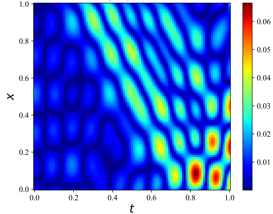
1D Wave (FLS) - Absolute Error
