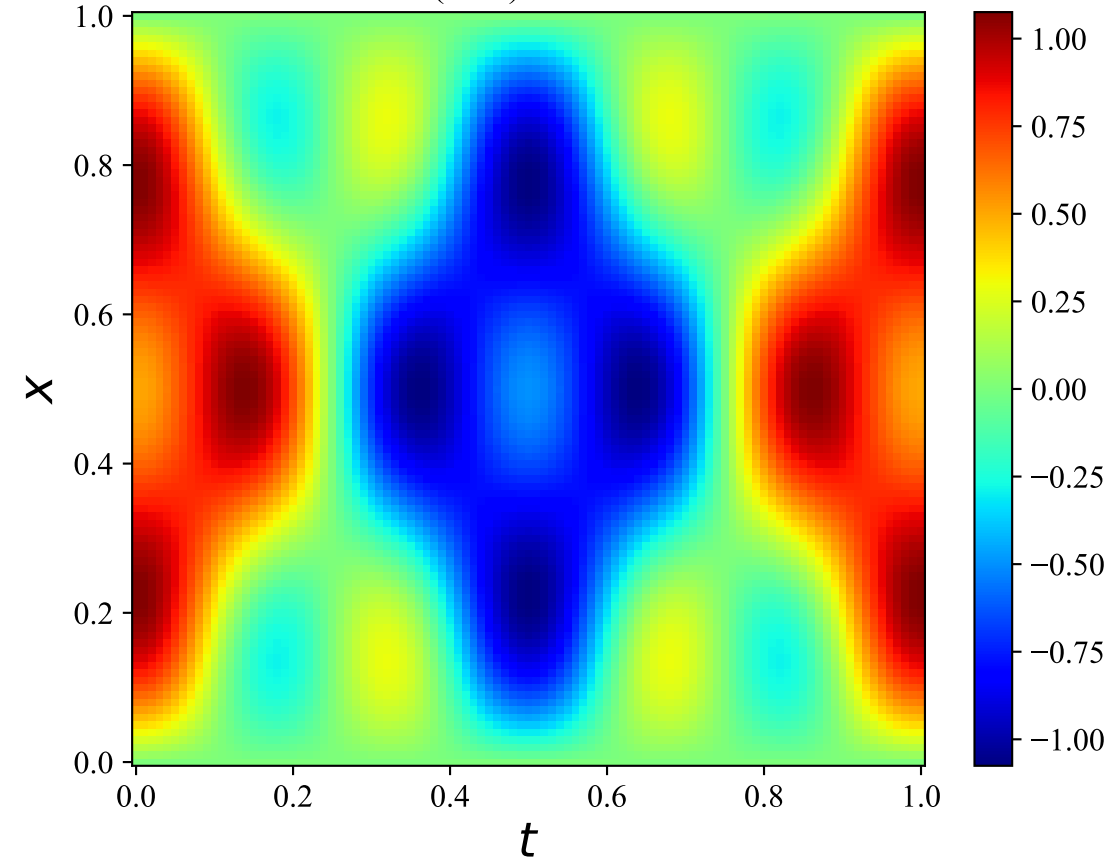
1D Wave (FLS) - Exact Solution
