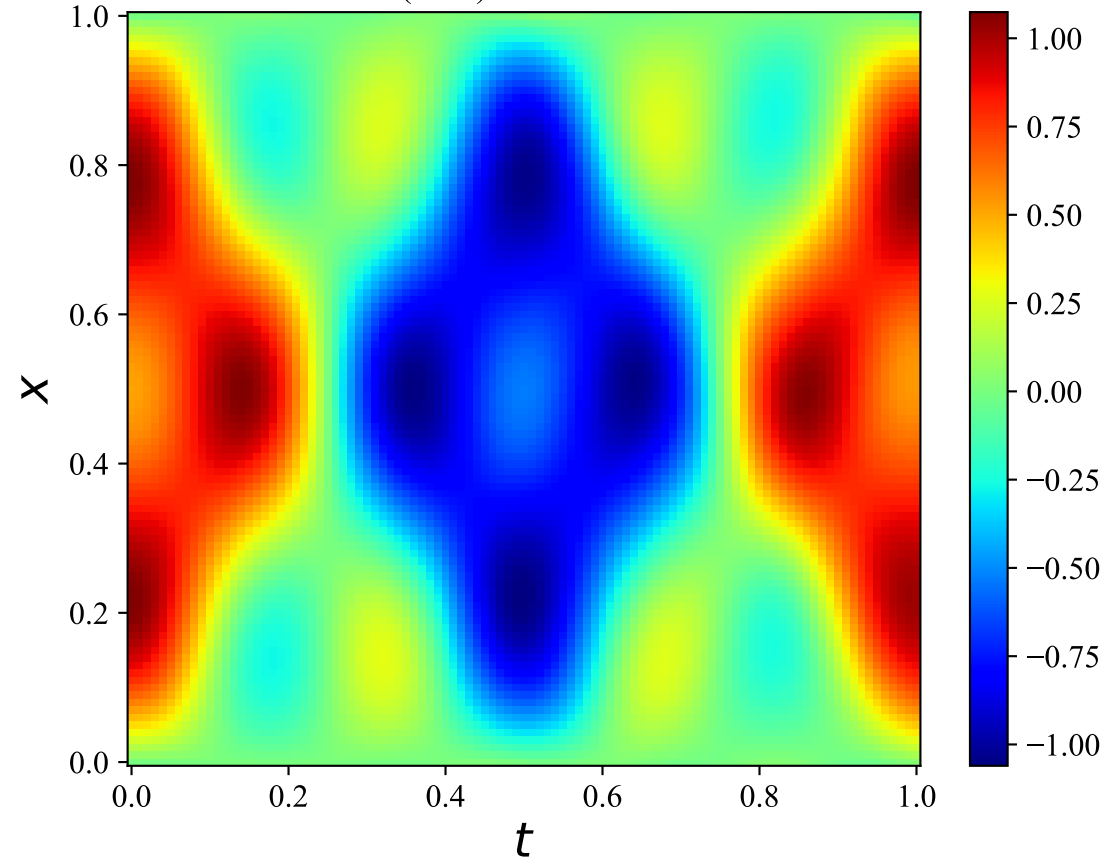
1D Wave (FLS) - Predicted Solution
