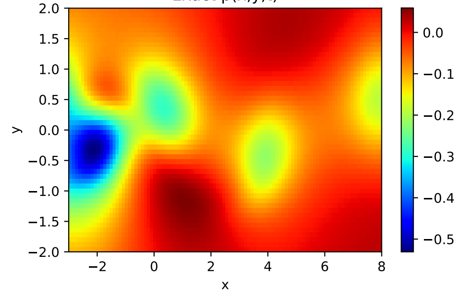
Exact p(x,y,t)
