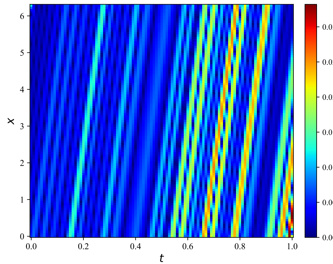
PINNsFormer
