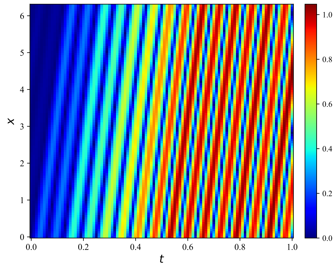
PINNsFormer
