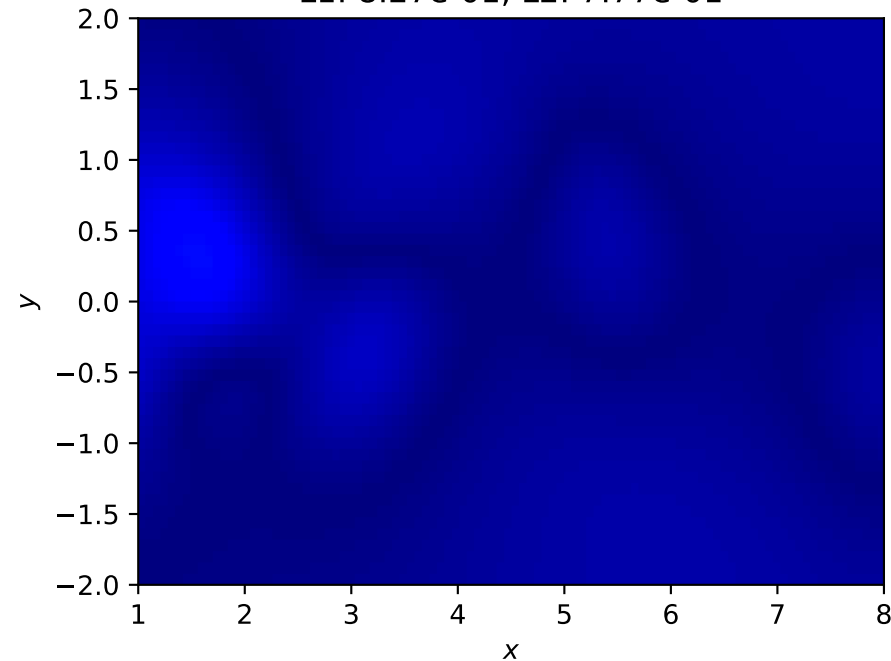
NS Pressure Error (PINNsFormer) L1: 8.27e-01, L2: 7.77e-01
