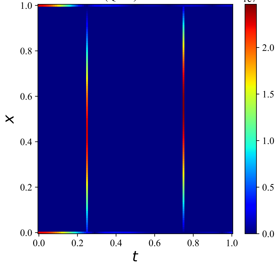
1D Wave (QRes) - Relative Error
