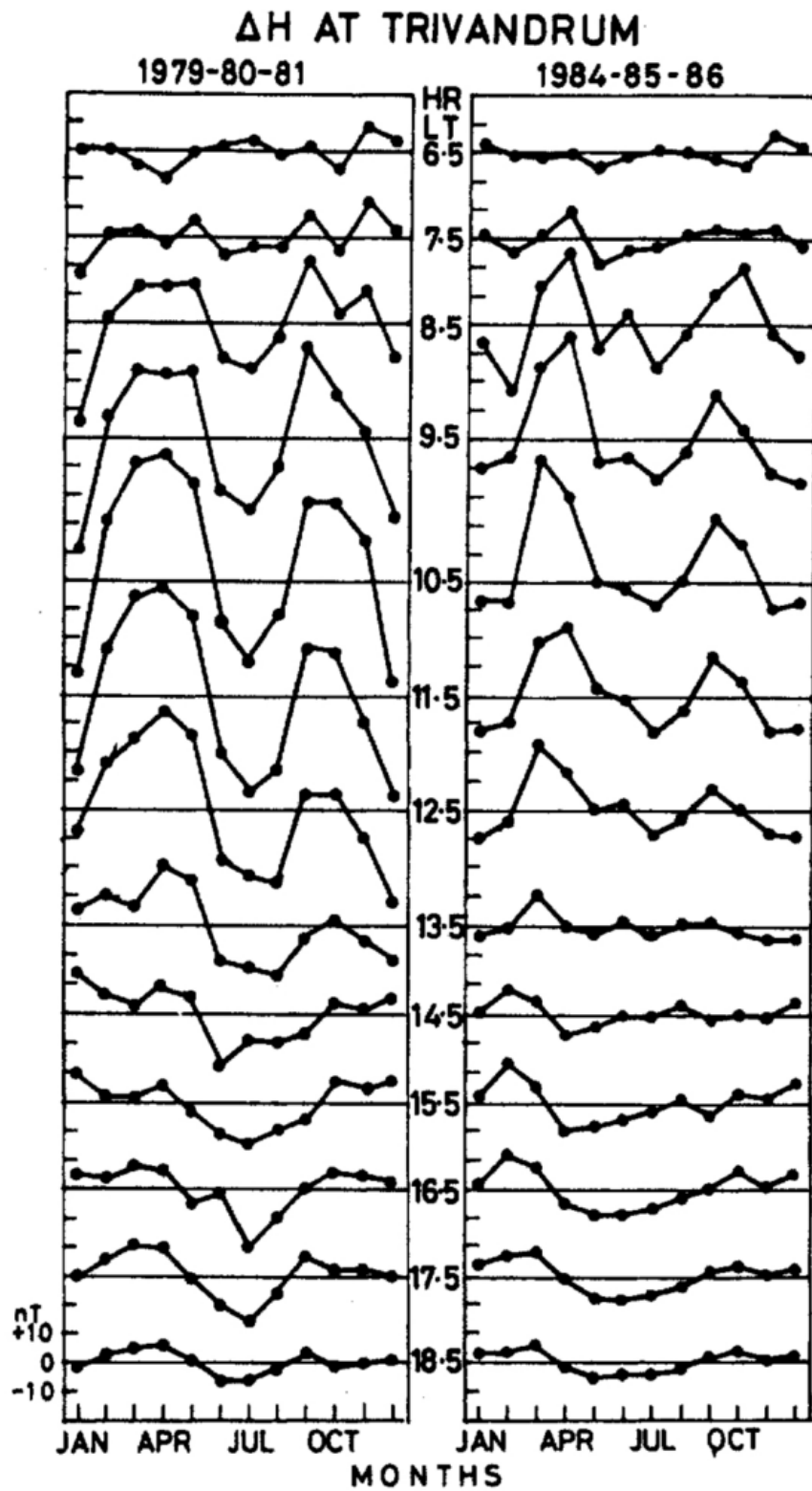
図2 Seasonal variations of Sq current system (Rastogi et al. 1994より引用).
