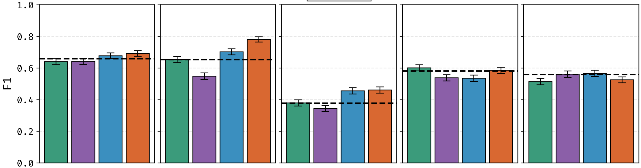
Qwen2.5-7B-Instruct
