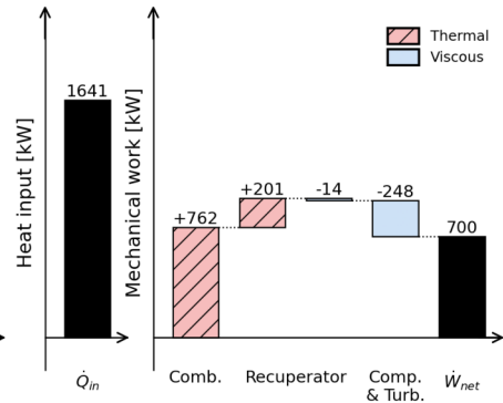
Aircraft level optimum \eta = 42.7\%
