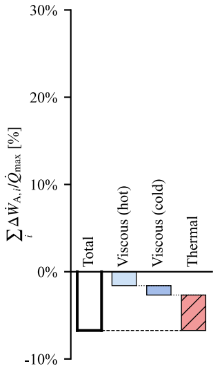
Classical Availability
