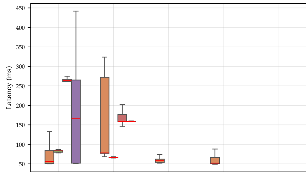
Latency by Client and Server Version (SlowAccept)
