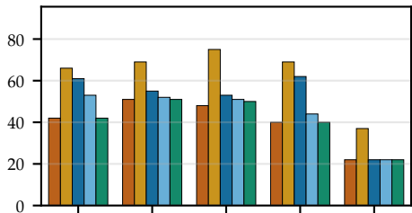
P95 Latency
