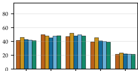
P10 Latency
