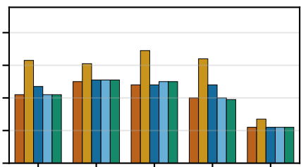
P99 Latency
