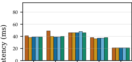
P95 Latency
