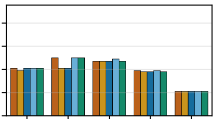
P90 Latency
