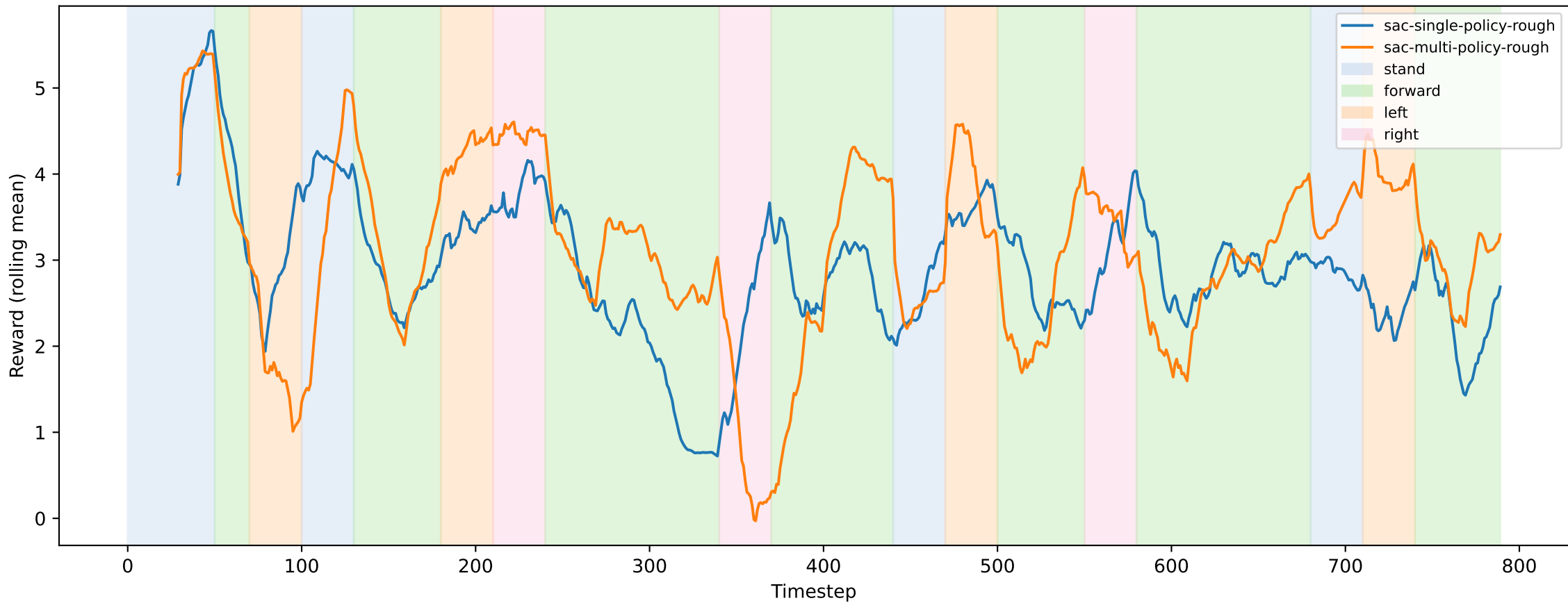
Average reward over time (window=30)
