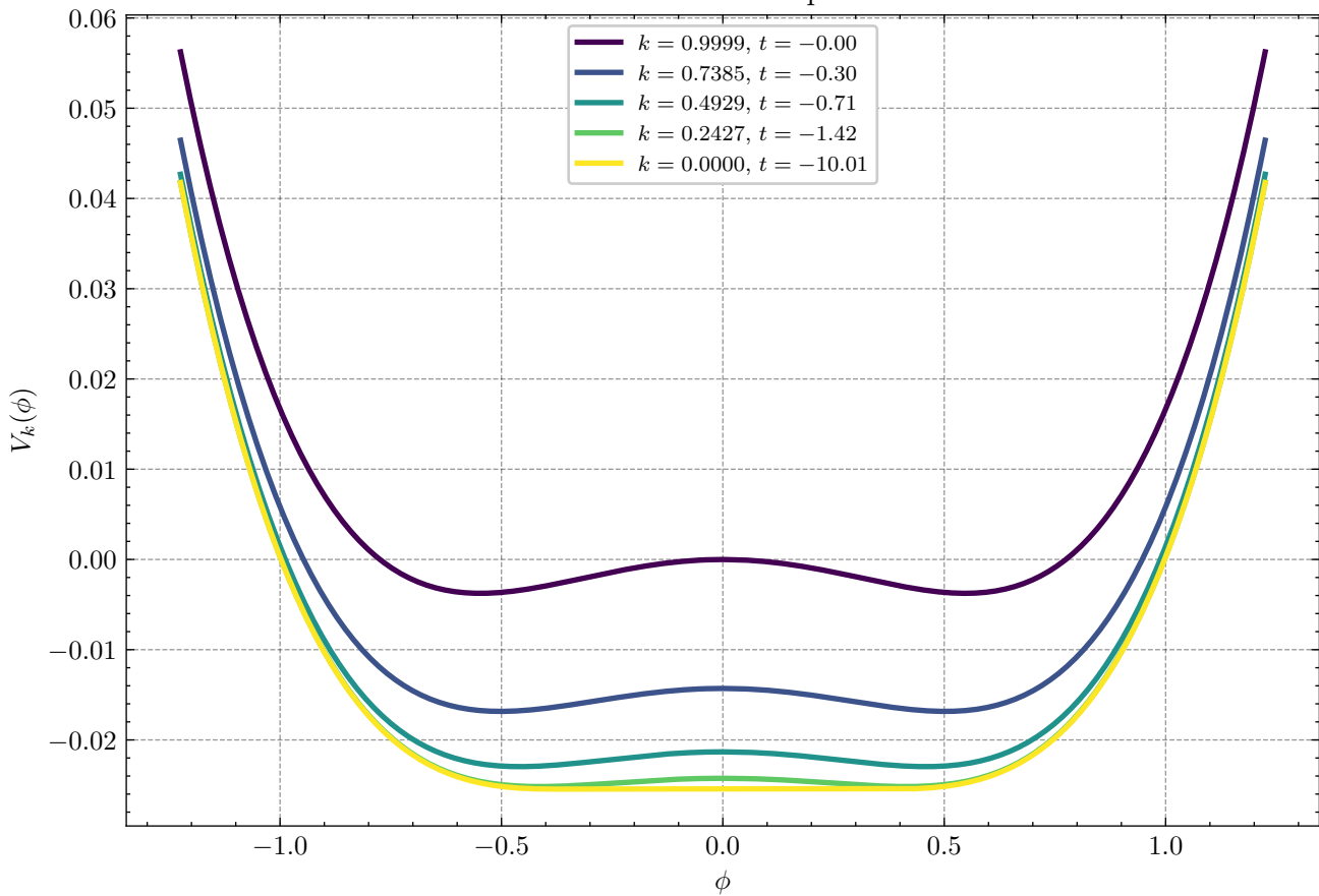
Flow of the effective potential
