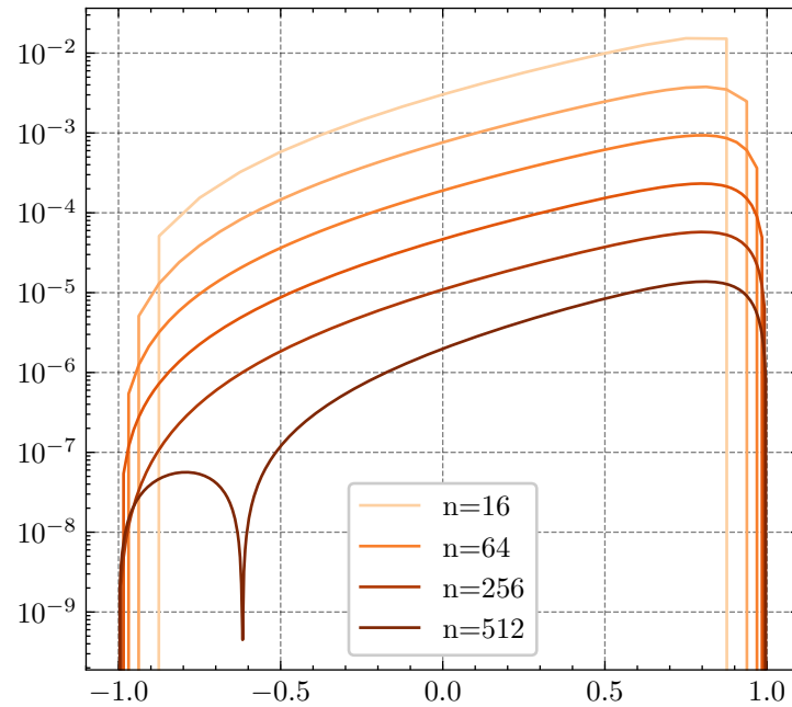
Pointwise error
