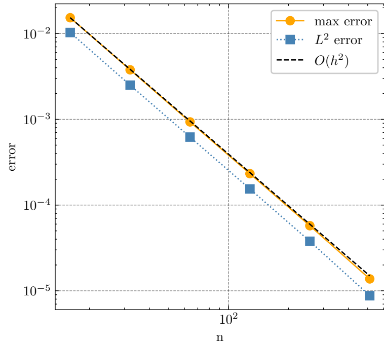
Convergence
