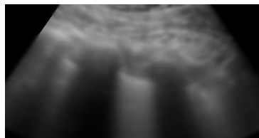
FIGURE 4 – Perona-Malik
