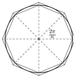
FIGURE 1. Unit circle with inscribed and circumscribed n -sided regular polygons, shown here with n = 8 .
