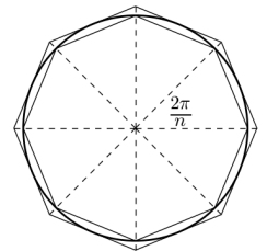
Figure 1: Unit circle with inscribed and circumscribed n -sided regular polygons, shown here with n = 8 .
