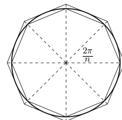
Figure 1: Unit circle with inscribed and circumscribed n -sided regular polygons
