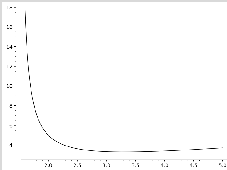
Fig: The graph of \phi to the right of 3/2 .
