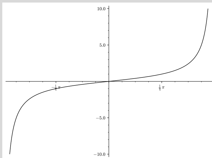
Fig: The plot of \tan(x)
