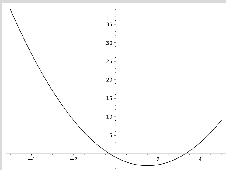
Fig: The plot of y^2 - 3y - 1
