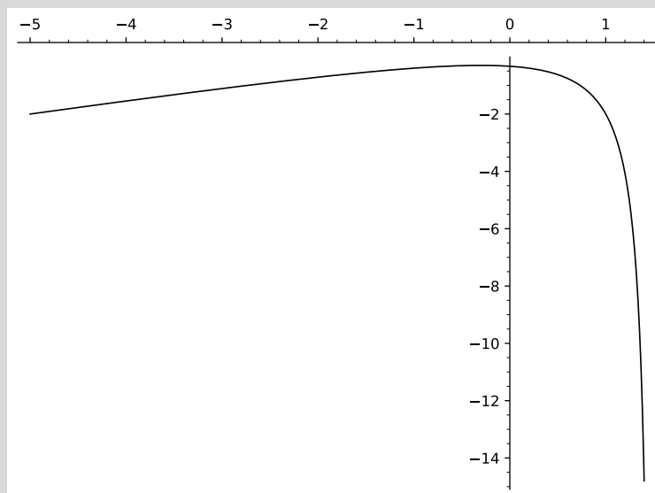
Fig: The graph of \phi to the left of 3/2 .
