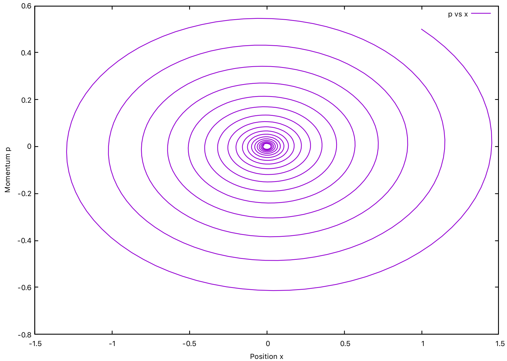
Sheriff CA2 Backward Euler
