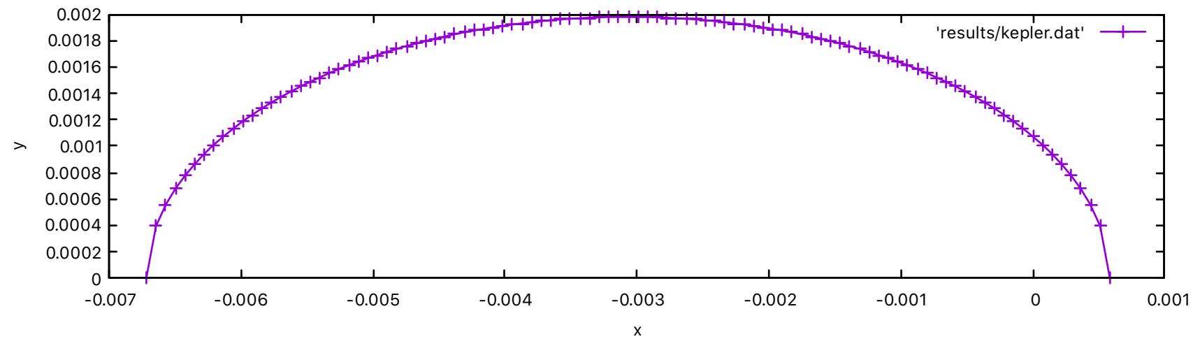
Kepler orbit
