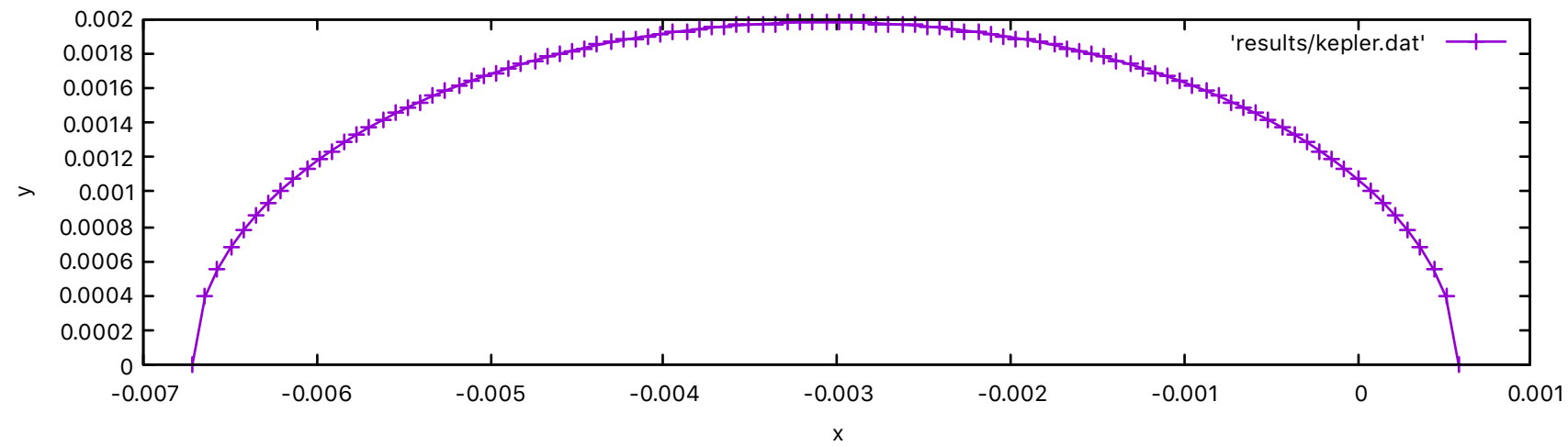
Kepler orbit
