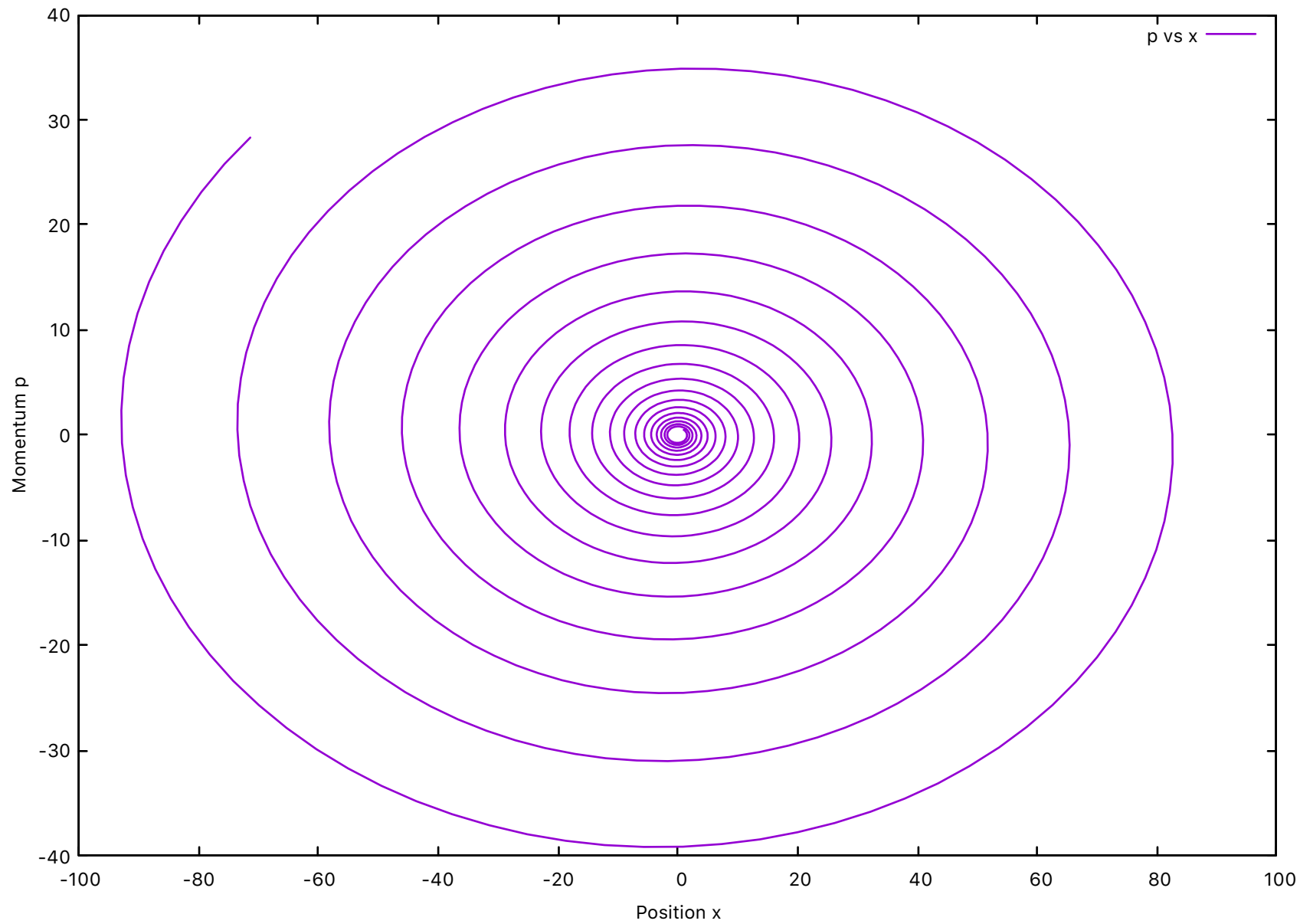
Sheriff CA2 Forward Euler
