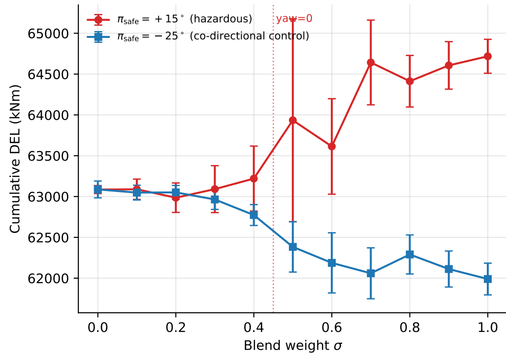
(a) Cumulative DEL vs \sigma
