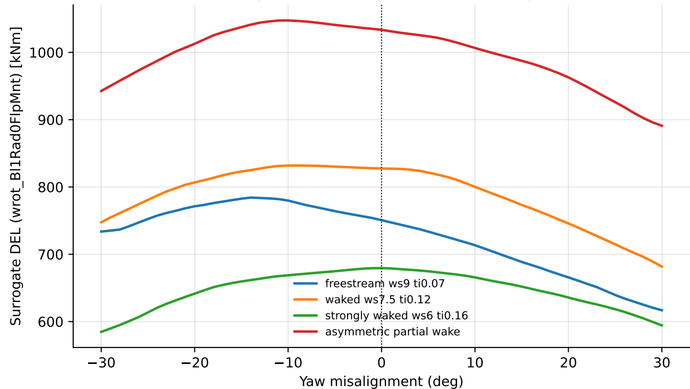
DEL vs yaw at fixed inflow (DLC12 surrogate)
