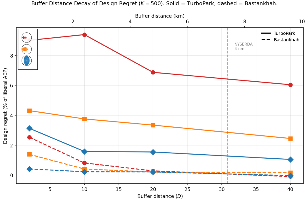
Figure 10. Regret vs. buffer distance at K = 500 , expressed as % of liberal AEP. The NYSEDA 4 nmi recommendation is marked.
