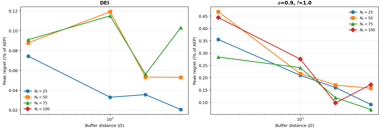
Figure C1. Peak regret vs. buffer distance at four target-farm sizes N_t \in \{25, 50, 75, 100\} . Neighbor is identical-copy throughout. Variation across N_t is at the same scale as multistart noise; no monotone trend in N_t is visible.
