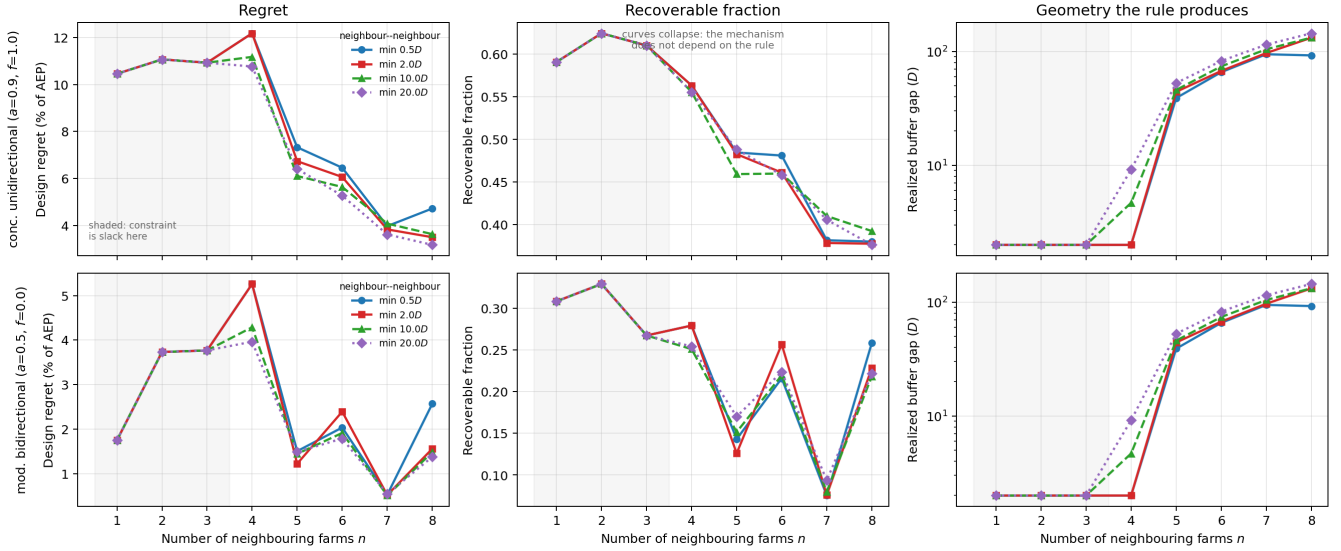
Figure E1. Sensitivity to the inter-neighbor minimum boundary gap (TurboPark, FunWake schedule, K = 500 , requested buffer 2D ). Right column: the geometry each rule produces, which differs by up to 4.6\times . Middle column: the recoverable fraction, on which the curves collapse. Shaded region: n \leq 3 , where the rule is slack and all settings coincide.
