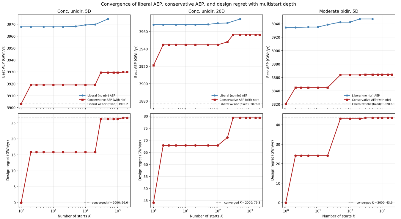
Figure 3. Convergence of design regret with multistart depth K (baseline schedule). Dashed gray: converged value ( K = 2000 ). All configurations stabilize by K \approx 500 under this optimizer configuration; see Fig. 4 for the schedule- and signal-size-dependence of this statement.
