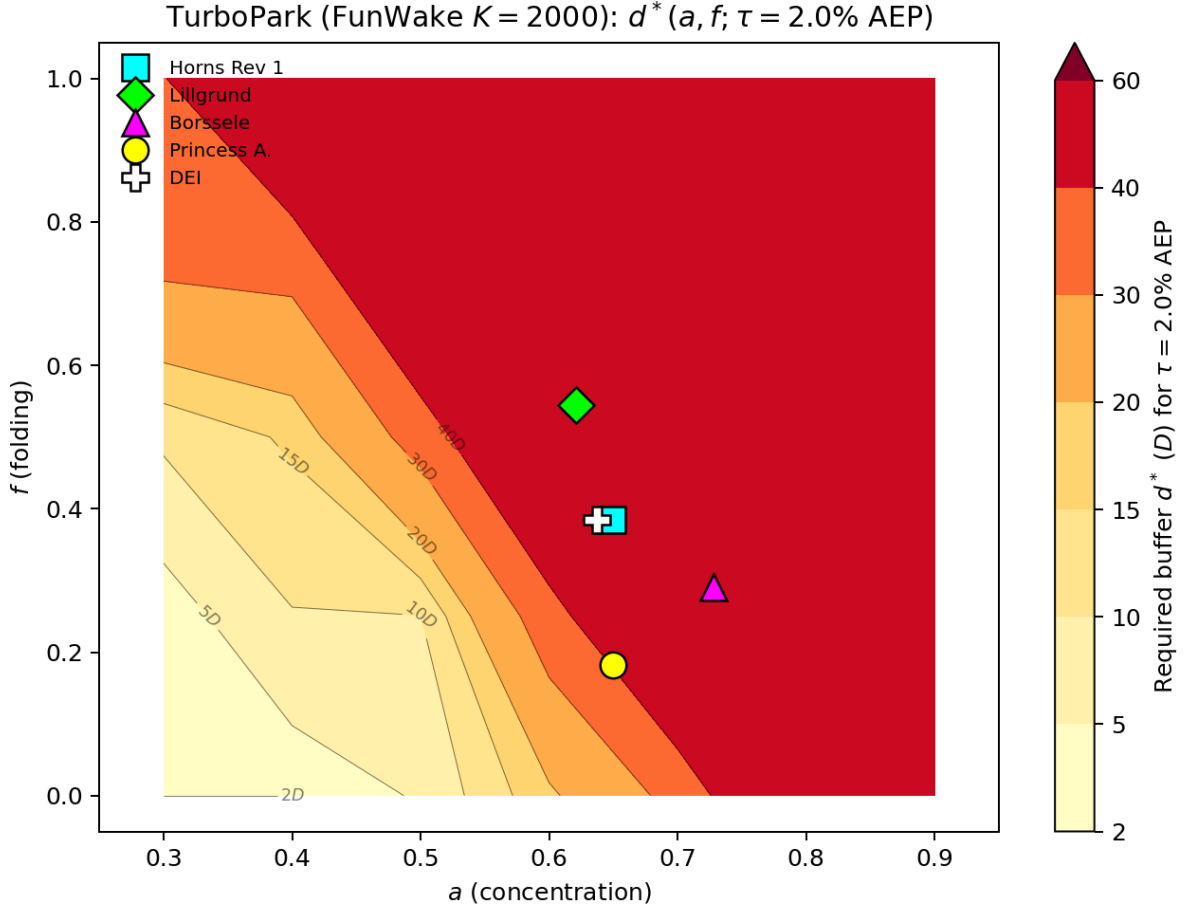
Figure 8. TurboPark. Required buffer d^*(a, f) at \tau = 2.0\% \text{ AEP} under TurboPark ( A = 0.04 , TI = 0.06 ; K = 2000 , FunWake schedule). Note the threshold is 10\times higher than Fig. 7, because TurboPark’s slower wake recovery raises realistic-scenario regret by one to two orders of magnitude. The threshold is unmet within the swept range ( d^* > 40D ) over most of the shape space, including the region containing all five fitted real sites: interpolated requirements run from \sim 42D (Princess Amalia, most bidirectional) to \sim 60D (Lillgrund, most unidirectional), i.e. 10–14 km.
