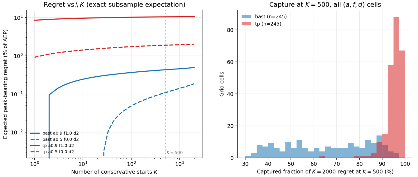
Figure 4. Multistart convergence computed exactly from stored per-start AEPs (FunWake schedule). Left: expected peak-bearing regret vs. start budget K for representative high- and low-regret cells (exact subsample expectation; no bootstrap noise). Right: fraction of the K = 2000 regret captured at K = 500 across all 245 buffer-table cells per wake model. TurboPark (red) is converged to within a few percent at K = 500 ; Bastankhah (blue), whose regret signal sits near the multistart noise floor, is not converged even at K = 2000 .
