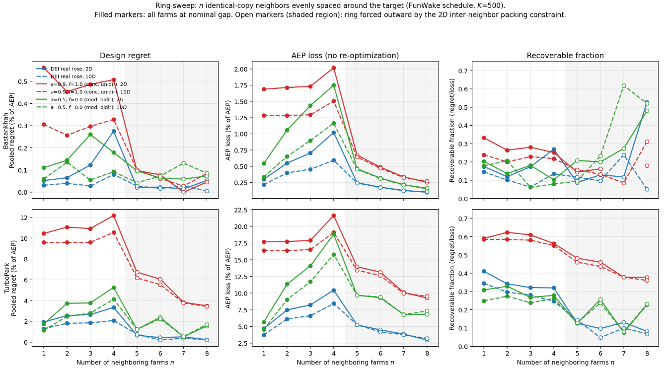
Figure 16. Ring sweep: n identical-copy neighbors evenly spaced around the target, starting from the prevailing upwind bearing (FunWake schedule, K = 500 ). Columns: pooled regret, AEP loss of the liberal layout, and their ratio (recoverable fraction). Rows: Bastankhah (top), TurboPark (bottom). Filled markers: all farms at the nominal boundary gap. Open markers (shaded region): the 2D inter-neighbor packing constraint forces the ring outward, so realized gaps exceed the nominal value.
