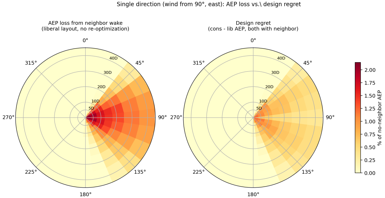
Figure A1. Single-direction validation case (wind exclusively from 90°): AEP loss (left) vs. design regret (right). Downwind bearings have zero regret as required by physics.
