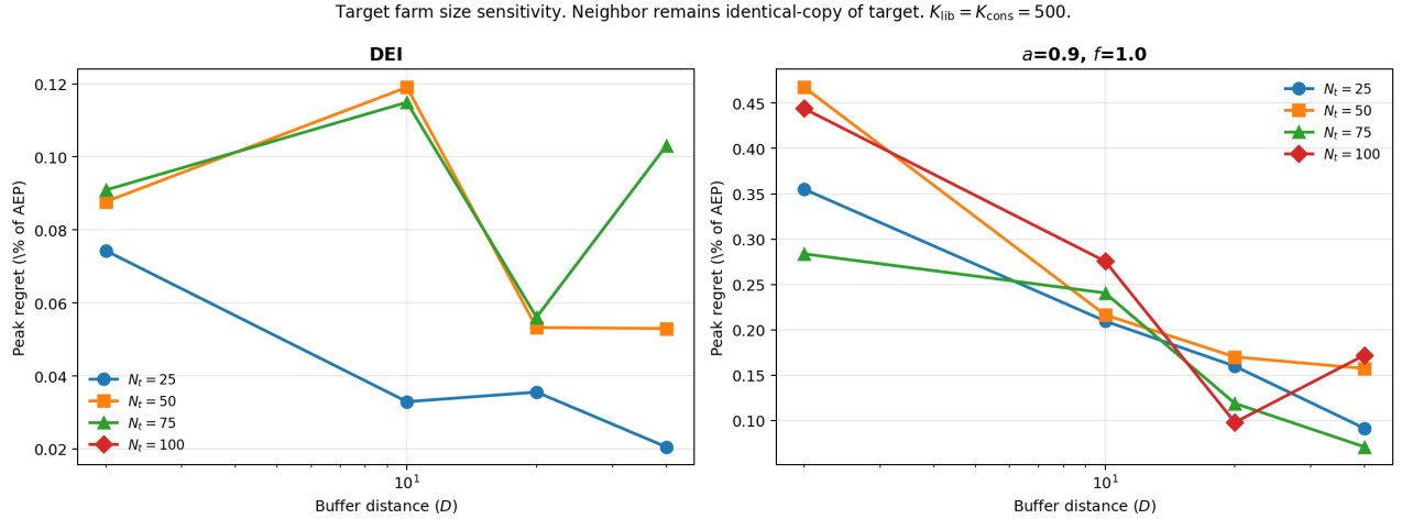
Figure C1. Peak regret vs. buffer distance at four target-farm sizes N_t \in \{25, 50, 75, 100\} . Neighbor is identical-copy throughout. Variation across N_t is at the same scale as multistart noise; no monotone trend in N_t is visible.
