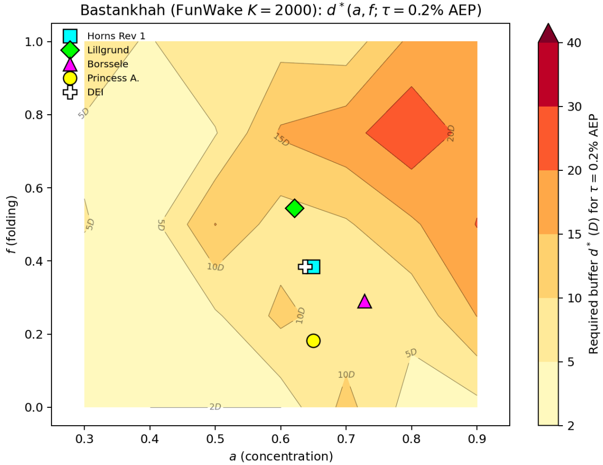
Figure 7. Bastankhah. Required buffer d^*(a, f) at \tau = 0.2\% \text{ AEP} ( K = 2000 , FunWake schedule). Markers: fitted real-site placements (Horns Rev 1, Lillgrund, Borssele, Princess Amalia, DEI). The five fitted real-site placements require d^* \approx 8\text{--}9D ( \sim 2 \text{ km} ) at this threshold.
