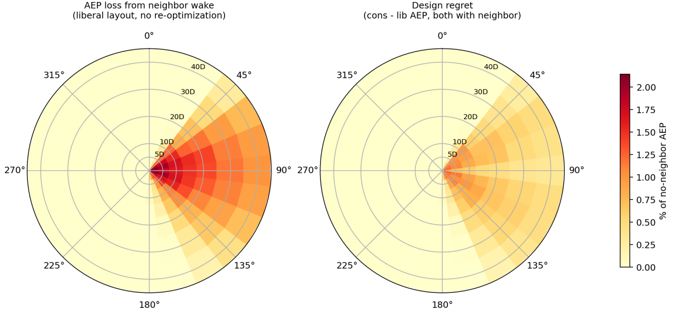
Figure A1. Single-direction validation case (wind exclusively from 90°): AEP loss (left) vs. design regret (right). Downwind bearings have zero regret as required by physics.
