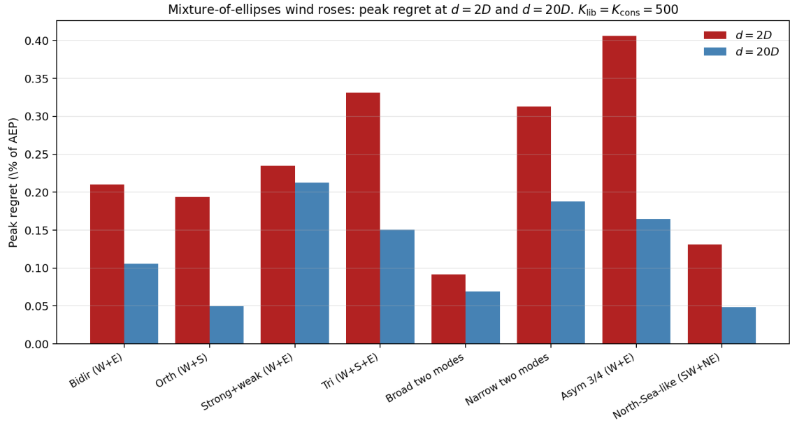
Figure B1. Peak regret for eight mixture-of-ellipses wind roses at d = 2D (red) and d = 20D (blue). All values stay within the single-rose envelope.
