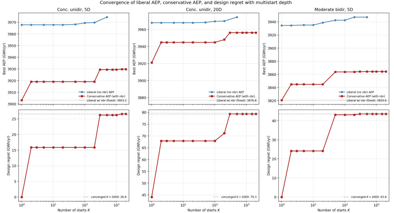
Figure 3. Convergence of design regret with multistart depth K (baseline schedule). Dashed gray: converged value ( K = 2000 ). Most of the gain is realised by K \approx 500 , but four of the six configurations step up again beyond it (Table 1); see Fig. 4 for the schedule- and signal-size-dependence of this statement.
