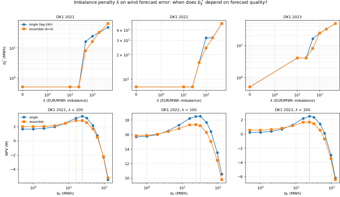
Figure 10: Imbalance-penalty sweep (DK1, 5-MW-peak wind + 1-MW battery, corrected settlement). Top row: b_E^* vs \lambda for single-forecast (blue circles) and K=4 multi-lag ensemble (orange squares) policies; argmax invariance holds at \lambda \leq 10 in every year and the policies separate inside the divergence bands (e.g. single 32 vs ensemble 24 MWh at \lambda = 100 in 2022). Bottom row: NPV curves at \lambda = 100 ; dotted verticals mark each policy’s argmax. Ensemble dominates NPV at its argmax in every panel.
