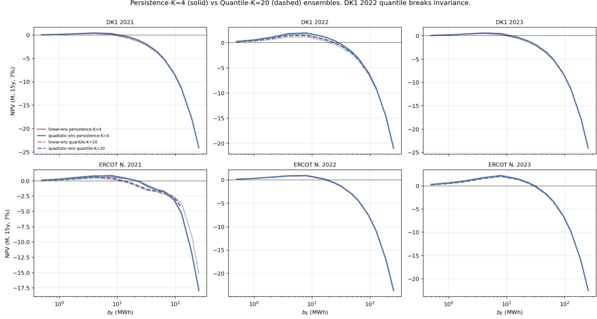
Figure 6: NPV vs b_E under persistence-K=4 (solid) and quantile-K=20 (dashed) ensembles. DK1 2022 (top centre) is the only panel where the linear-cost single-forecast argmax disagrees with the others under the richer quantile ensemble.
