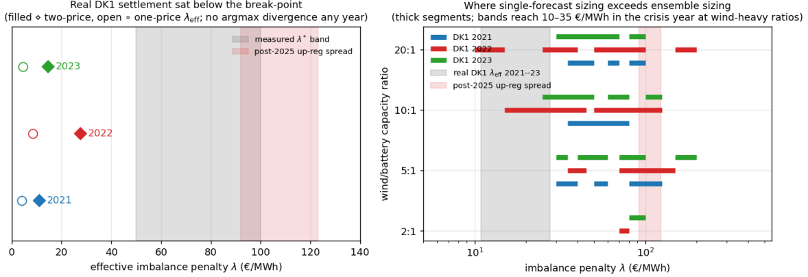
Figure 11: Real-settlement anchor for the break-point study. Left: effective penalty \lambda_{\text{eff}} of actual DK1 imbalance settlement (eSett) per study year, against the measured break-point band and the post-March-2025 mean up-regulation spread; no argmax divergence occurs under real settlement in any year. Right: \lambda ranges where the single-forecast policy sizes above the ensemble (thick segments, fine \lambda grid, corrected settlement), by wind/battery ratio and year; bands open at 25–35 EUR/MWh in normal years and reach 10–15 in the 2022 crisis year at wind-heavy ratios. Real 2021–2023 settlement (grey) overlaps the crisis-year bands at wind-heavy ratios — where real-settlement sizing indeed splits (8 vs 4 MWh) — and post-2025 spreads (red) sit deep inside the bands.
