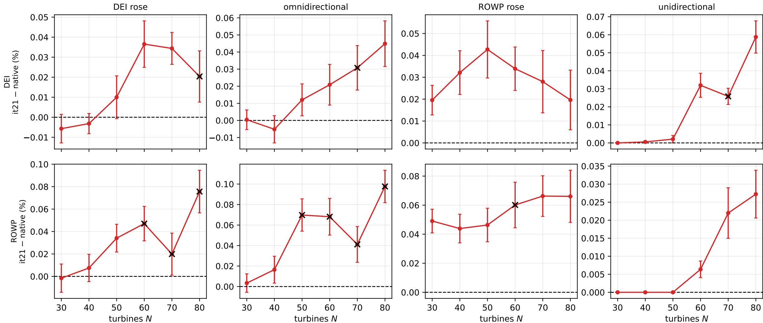
Generalization: feasible-paired-mean AEP advantage of it21 over native (30 seeds/cell; error bars = se; × = it21 feasibility < 100%)
