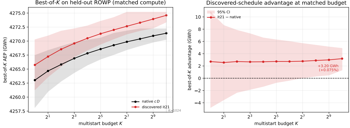
Figure 6: Best-of- K deployment comparison on the held-out ROWP farm at matched compute, bootstrapped from independent deep pools (native 4096 runs; discovered it21 2048 runs). Left : best-of- K AEP versus multistart budget K (median with 5–95th percentile band); the discovered schedule’s median sits above the native reference across budgets. Right : the best-of- K advantage (discovered – native) with a 95% bootstrap band; the median advantage is positive throughout, but the band excludes zero only near the calibrated budget K = 1024 , where the advantage is +3.2 GWh (+0.075%). The interval reflects best-of- K sampling variability only, conditional on the selected schedule and the ROWP pools.
