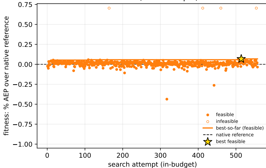
Claude (557 attempts)
