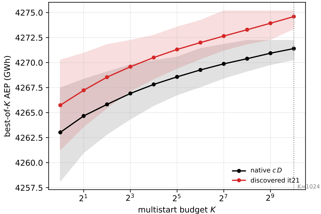
Best-of-K on held-out ROWP (matched compute)
