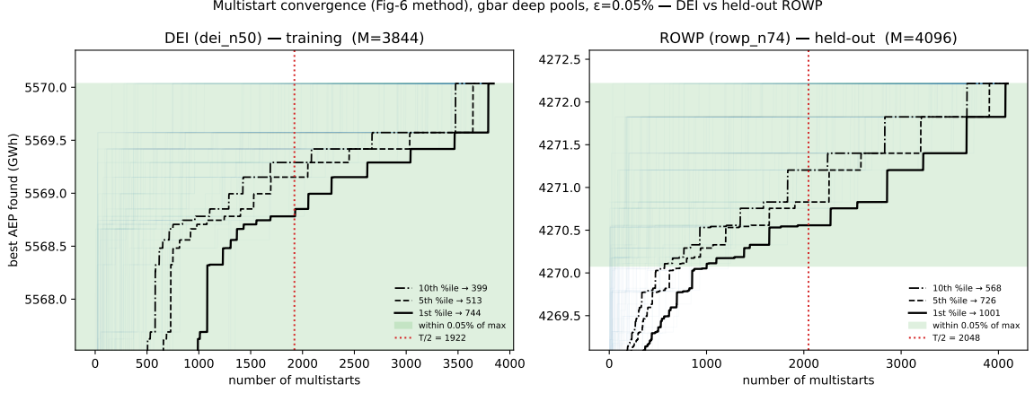
Figure 2: Shuffle-saturation convergence of the reference multistart on the DEI training farm (left) and the held-out ROWP farm (right), following Quick et al. (2026). Faint lines are individual shuffles of the pool; the black curves are the tenth-, fifth-, and first-percentile running maxima; the shaded band is within \epsilon = 0.05\% of the pool maximum, and the dotted vertical line is the half-pool budget M/2 . Each percentile reaches the band well inside M/2 on both farms; the held-out ROWP farm (sparser near-optimum basin) requires more starts than the training farm.
