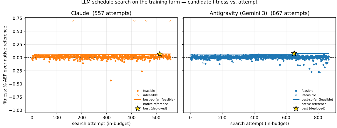
Figure 3: Schedule search on the training farm for two mutation engines (Claude, left; Antigravity/Gemini 3, right). Each point is a candidate schedule proposed by the LLM and scored by the fixed skeleton; filled points are feasible on every seed, hollow points are infeasible; the solid line is the best feasible fitness so far; the dashed line is the native reference (0%); the star marks the best (deployed) schedule. The best-so-far improves only \approx 0.05\text{--}0.09\% over the native reference, and the infeasible +0.7\% outliers are non-deployable layouts discarded by the feasibility gate.
