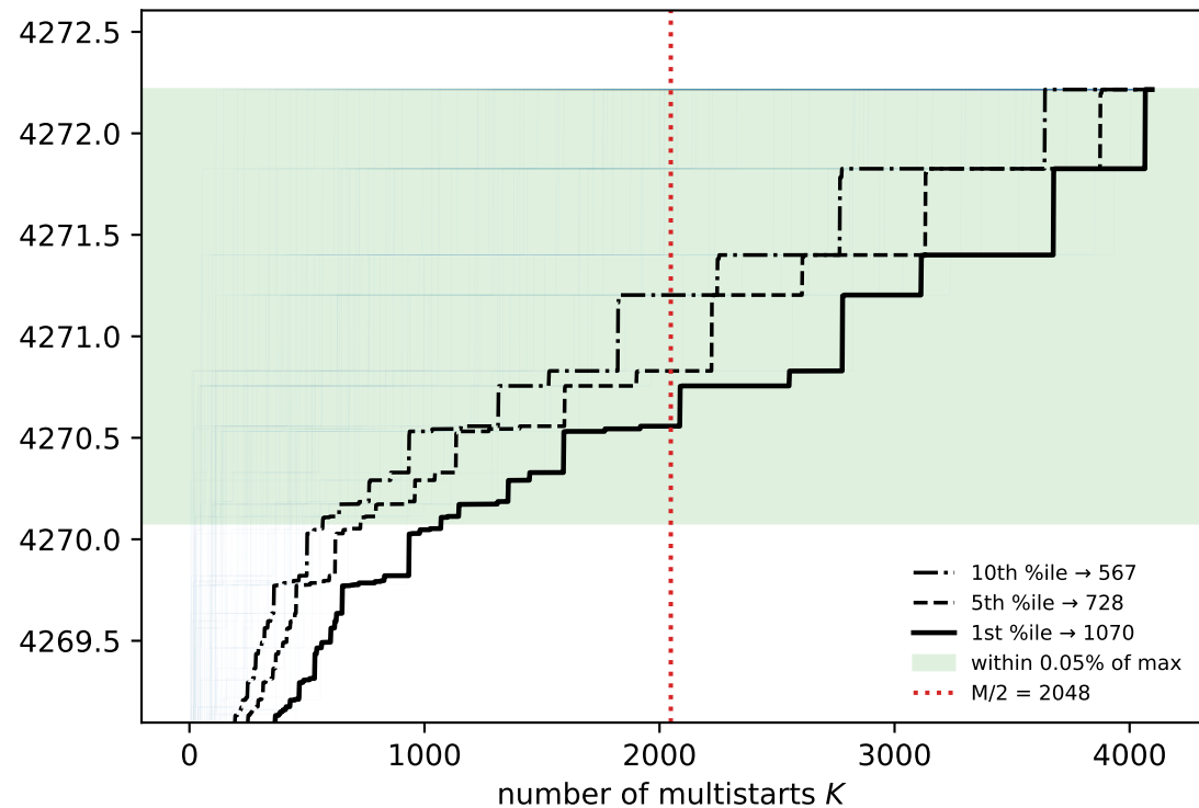
ROWP (rowp_n74) — held-out ( M = 4096 )
