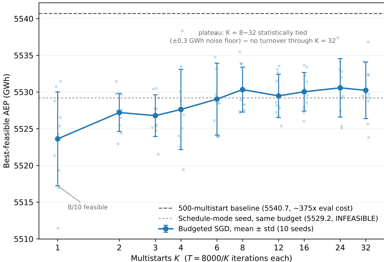
Equivalent-cost SGD frontier (8000 gradient evaluations, DEI farm)
