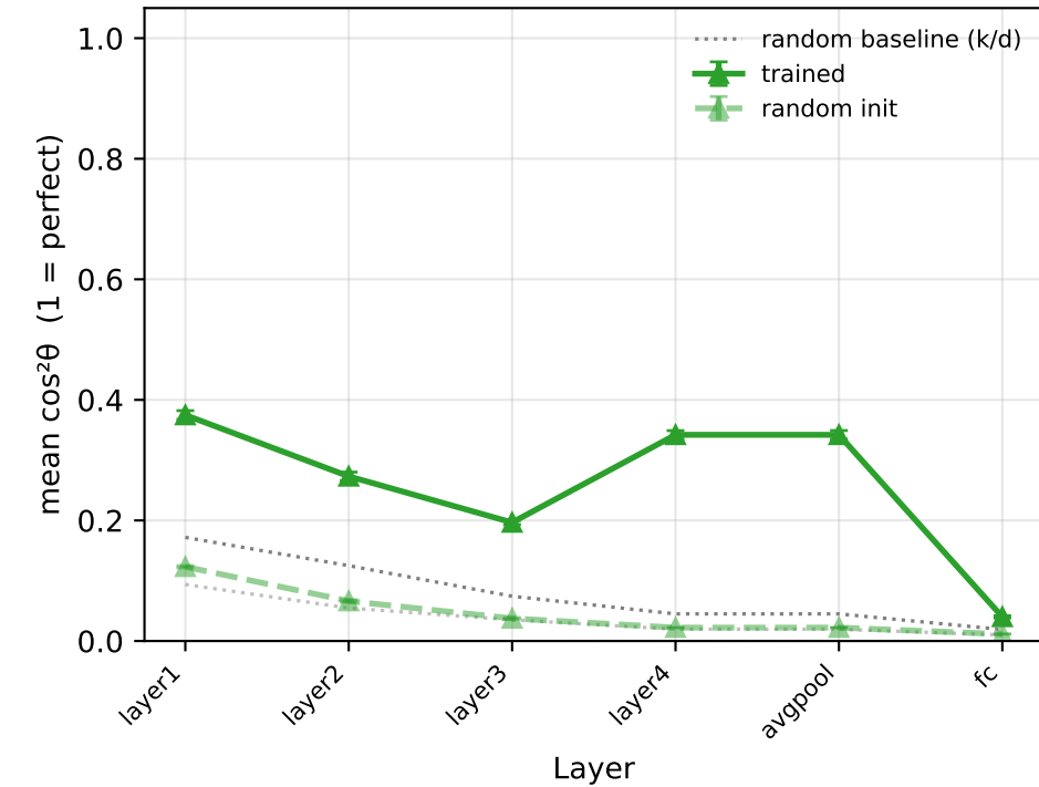
ResNet-18 — PCA vs AGOP alignment
