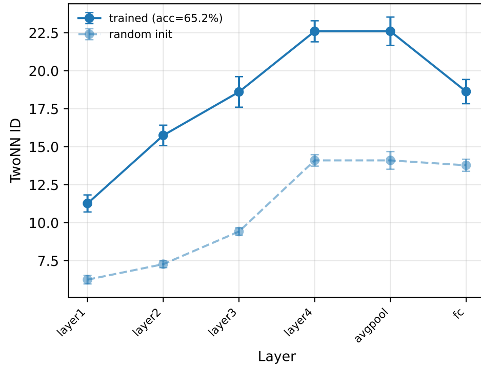
ResNet-18 — intrinsic dimension
