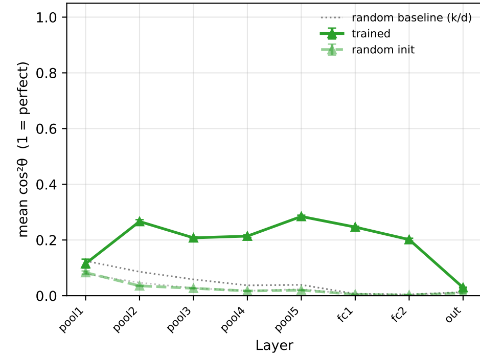
VGG-16 — PCA vs AGOP alignment
