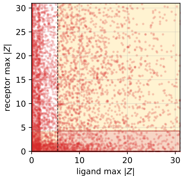
M1: purifying selection (strong on receptor) hit pattern: 14.8% of replicates
