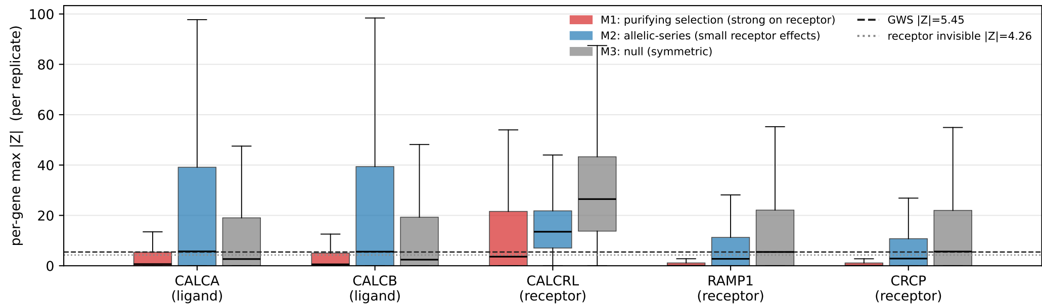
M1: purifying selection (strong on receptor) hit pattern: 14.8% of replicates
