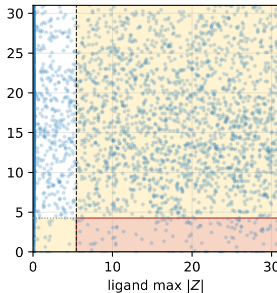
M2: allelic-series (small receptor effects) hit pattern: 3.5% of replicates
