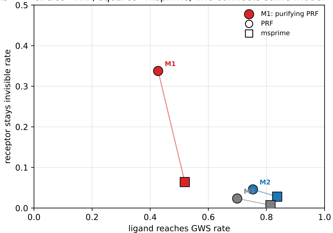
Component decomposition circles=PRF, squares=msprime; line connects same model
