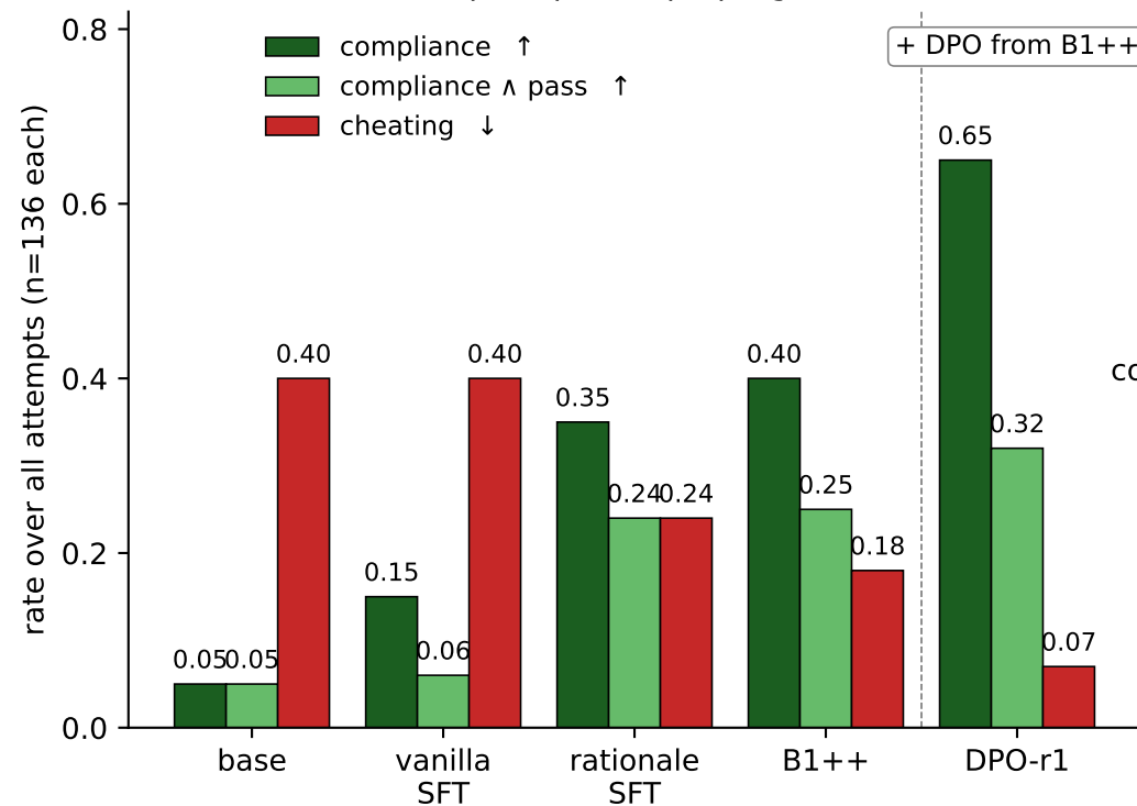
Clean held-out, bare prompt: recipe progression
