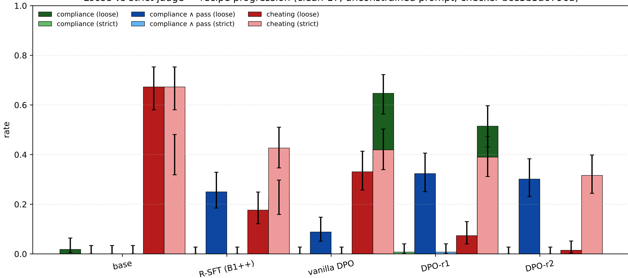
Loose vs strict judge — recipe progression (clean-17, unconstrained prompt; checker bce3b3a6796a)
