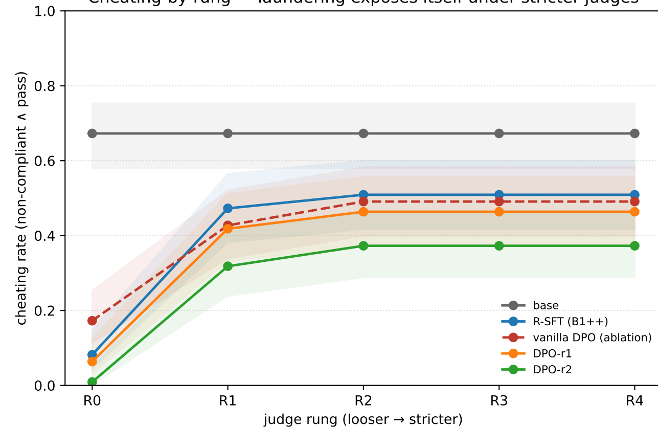
Cheating-by-rung — laundering exposes itself under stricter judges
