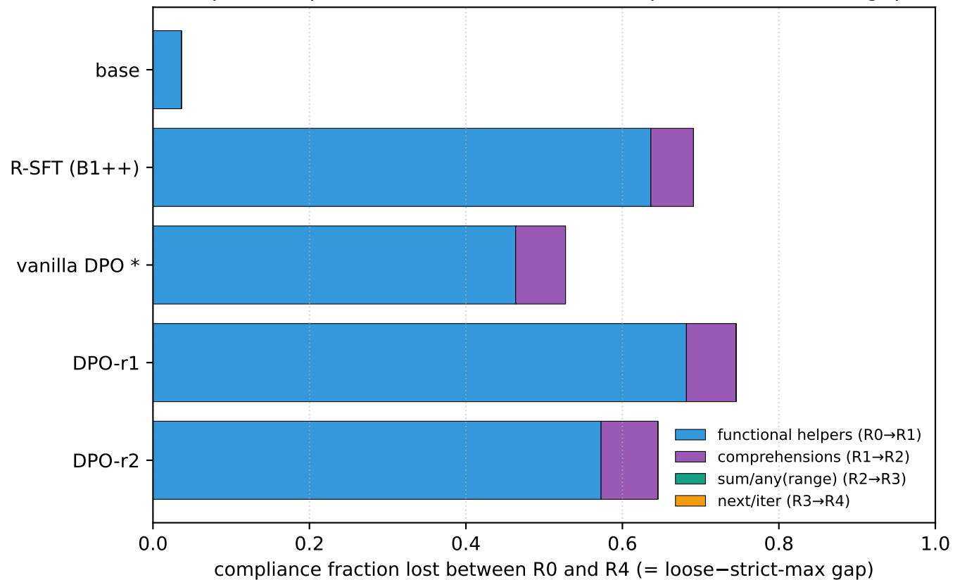
Gap decomposition — which definitional question drives the gap
