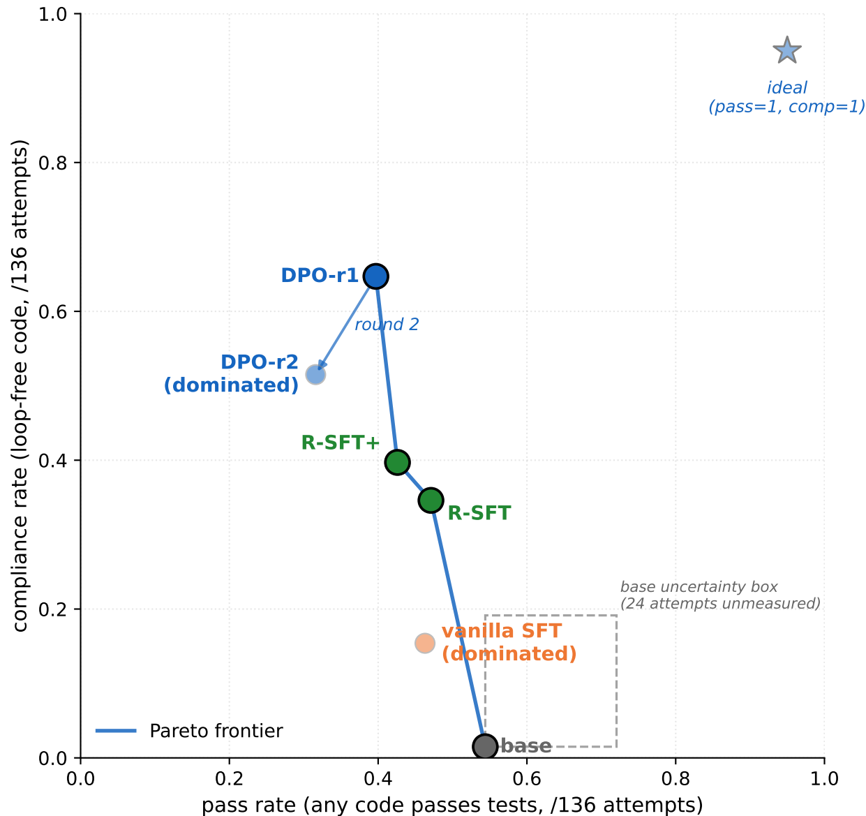
Pareto frontier on LCB clean: pass vs compliance
