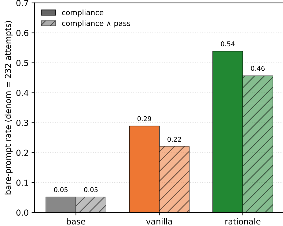
Held-out eval (29 problems combined, n=8, T=0.7)
