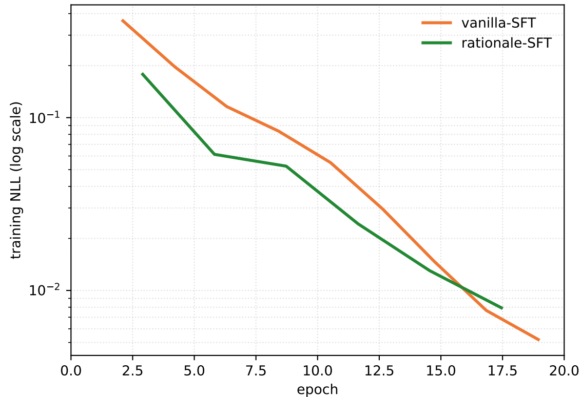
Training NLL — same recipe, same epochs
